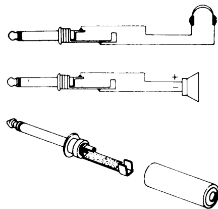
Headphone and external speaker connections
