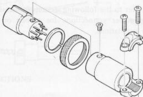
YM-37 MICROPHONE CONNECTIONS
