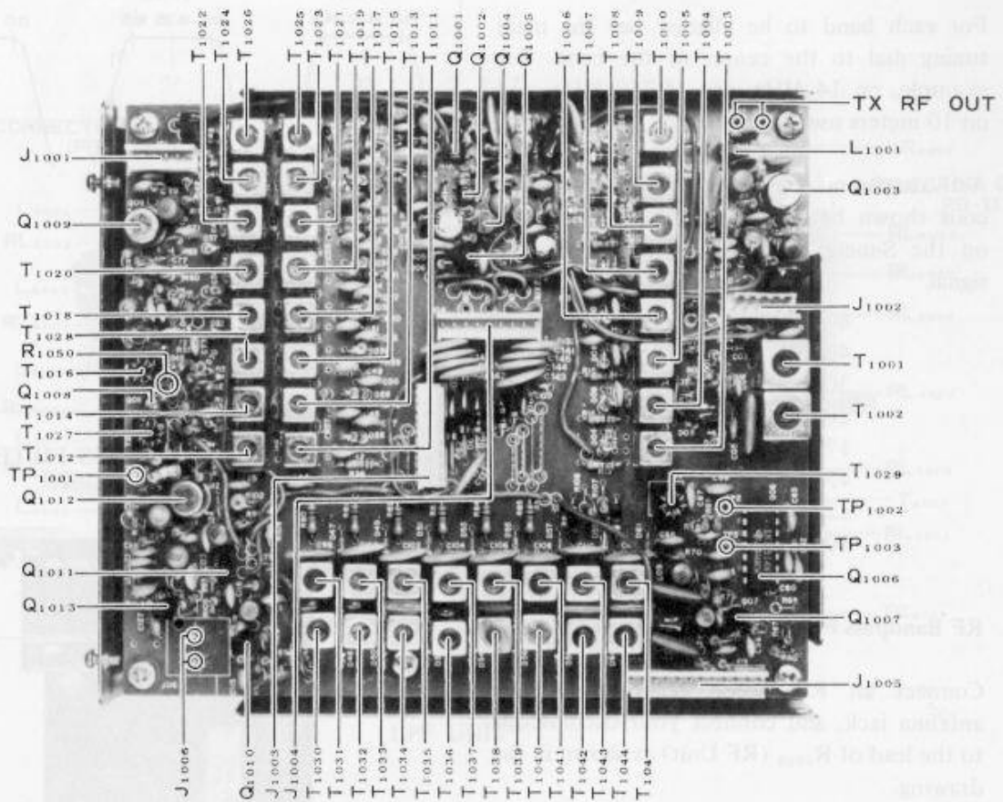
RF UNIT
