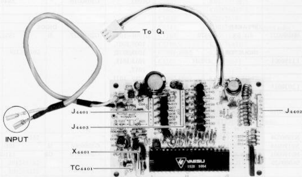
COUNTER UNIT
