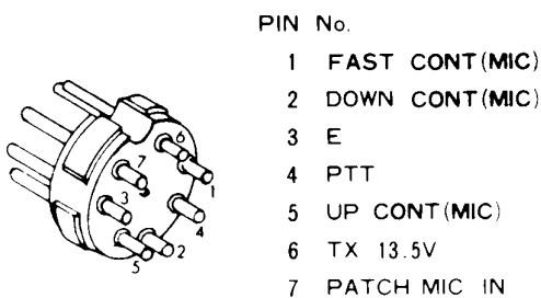
ACC Plug
