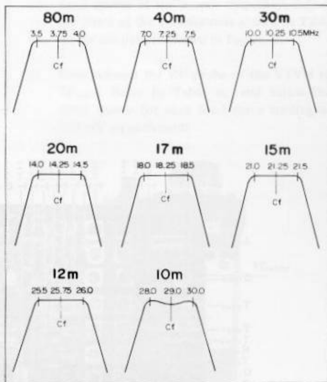
Figure 6 RF BANDPASS FILTER
