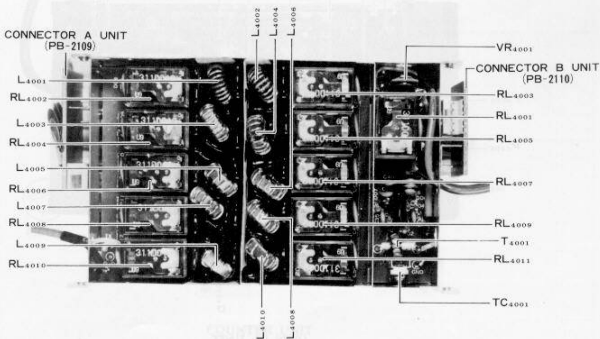
LPF UNIT
