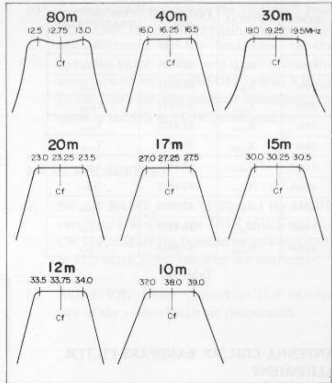
Figure 5 PREMIX BANDPASS FILTER
